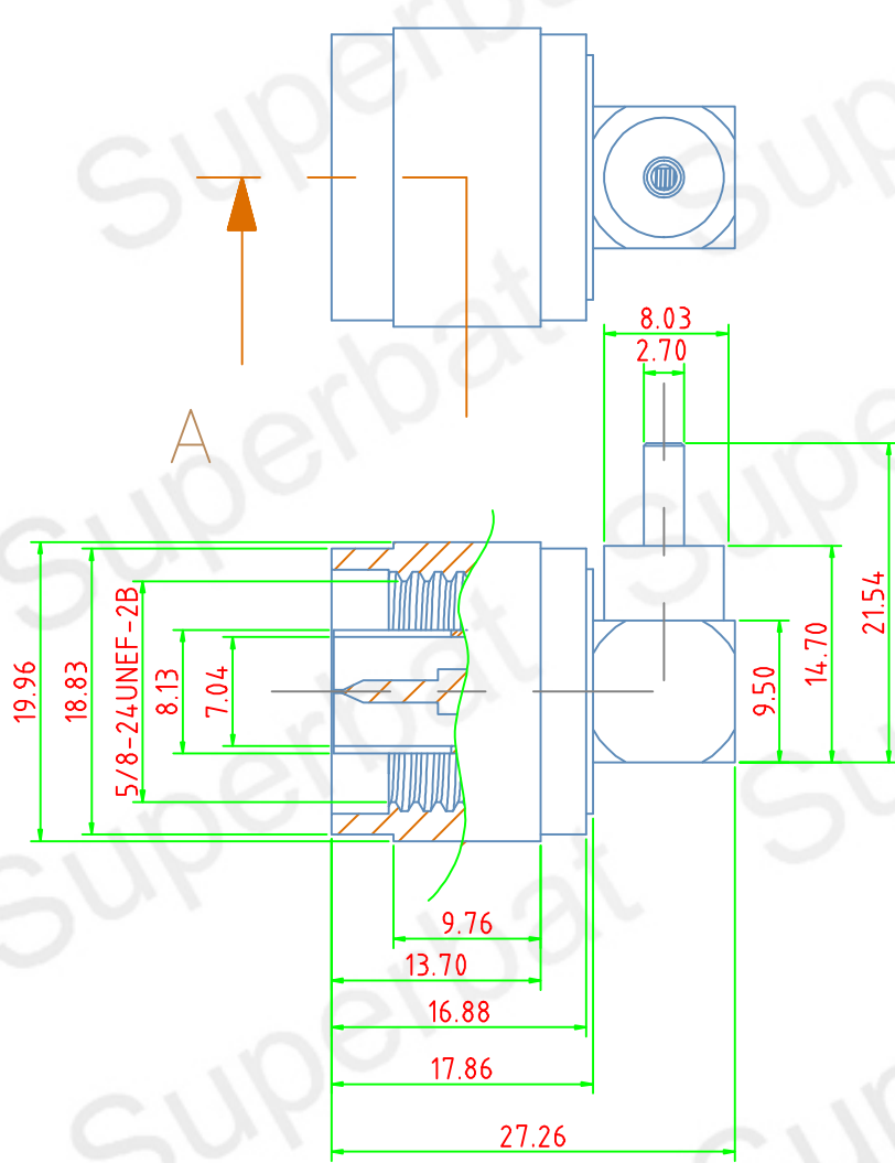
SECTION A—A
