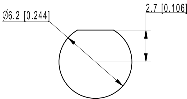
MILLED FLAT
