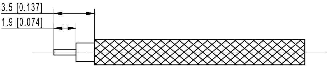
STRIPPING DIMENSIONS
