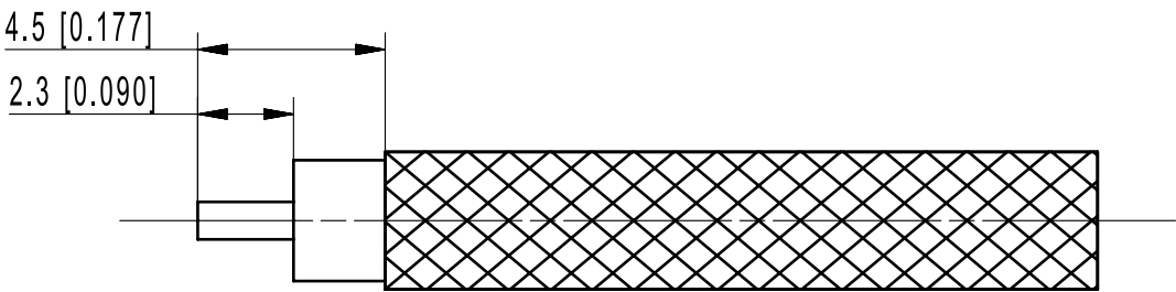
STRIPPING DIMENSIONS
