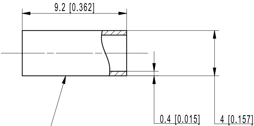
④ CRIMP SLEEVE
