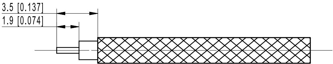
STRIPPING DIMENSIONS
