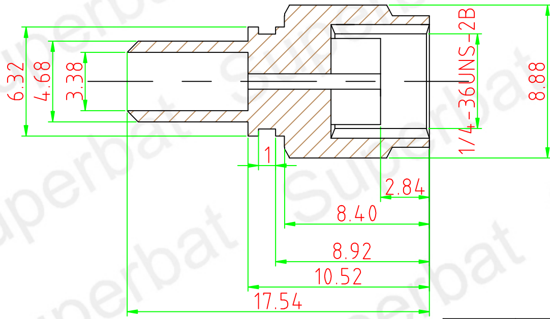
SECTION B-B
