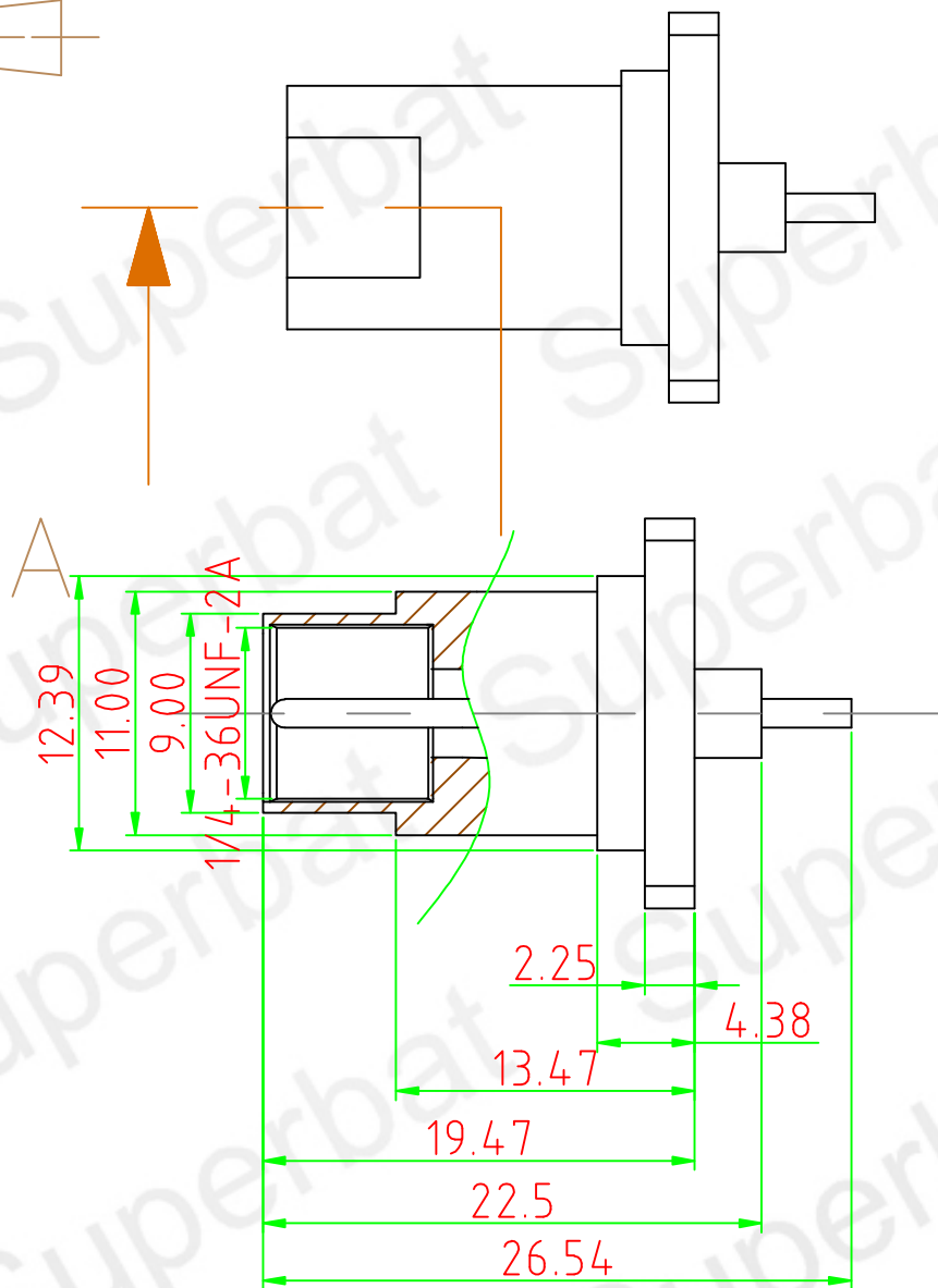
SECTION A—A
