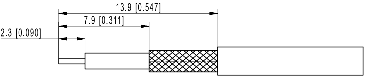
STRIPPING DIMENSIONS
