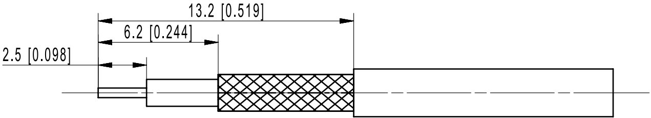
STRIPPING DIMENSIONS
