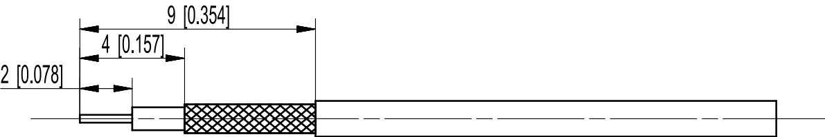
STRIPPING DIMENSIONS
