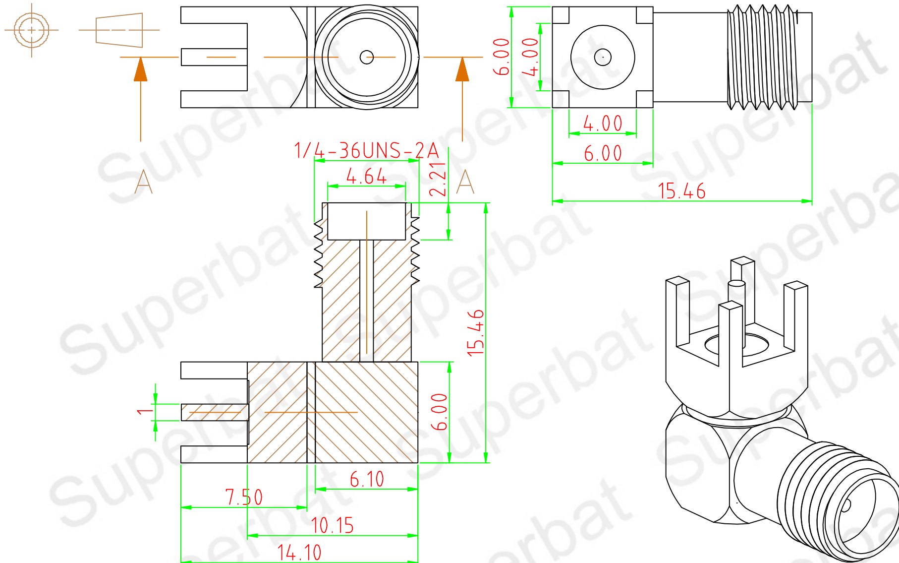
SECTION A—A
